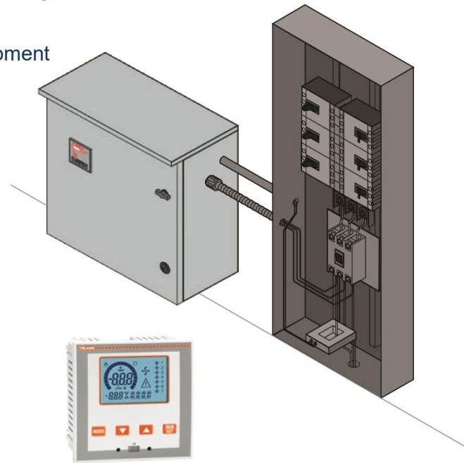
Digital Controller
